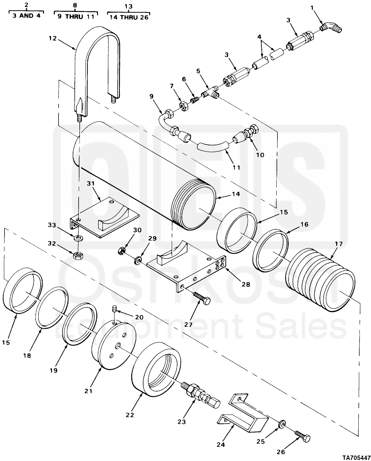
FIGURE 121. HYDRAULIC BRAKE ACCUMULATOR AND HOSES.
